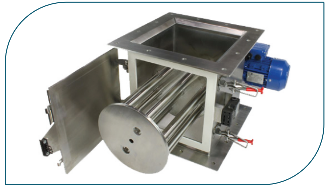
Rotary Magnet
